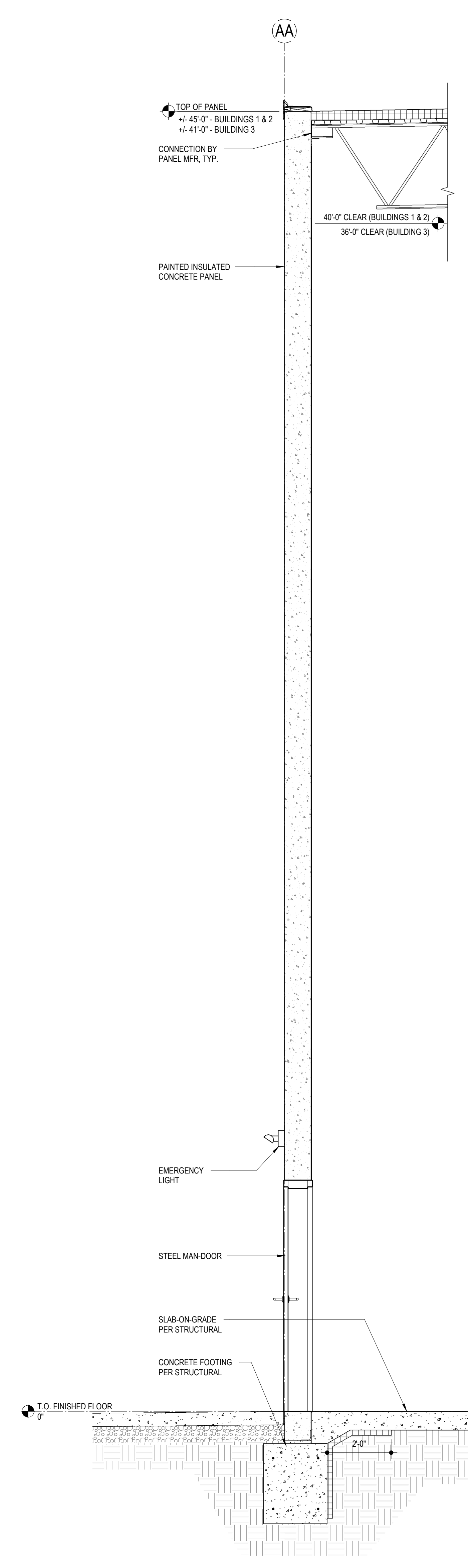
2 TYPICAL WALL SECTION AT MAN-DOOR AT GRADE 1/2" = 1'-0"
